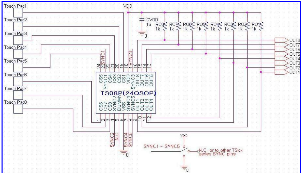
TS08P(24QSOP) Application Example Circuit
